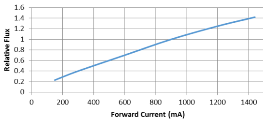
CDM-18 Relative Luminus Flux vs. Forward Current @ T_j=85^\circ\text{C}
