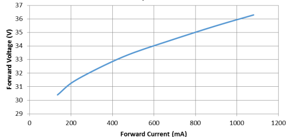
CDM-18 Forward Voltage vs. Forward Current @ T_j=85^\circ\text{C}
