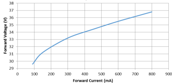
CDM-14 Forward Voltage vs. Forward Current @ T_j=85^\circ\text{C}
