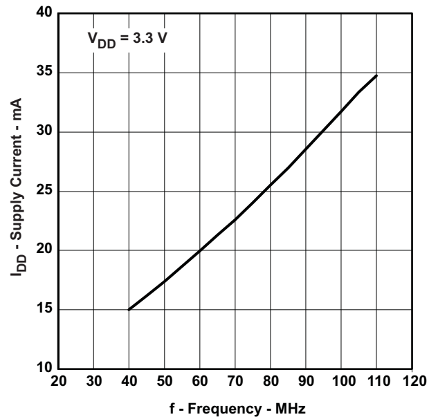
Figure 1. I_{DD} vs. Input Frequency, V_{DD} = 3.3 \text{ V}
