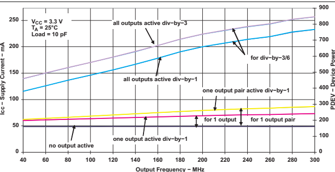
Figure 2. LVPECL Device Power Consumption vs Number of Active Outputs
