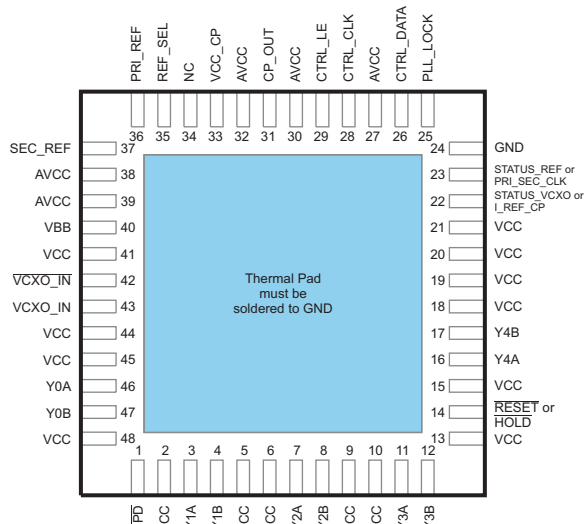
RGZ Package 48-Pin VQFN Top View
