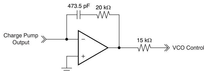
Figure 14. On-Chip PLL Loop Filter Topology
