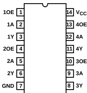
CD54HC126, CD54HC126 (CERDIP) CD74HC126, CD74HC126 (PDIP, SOIC) TOP VIEW
