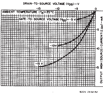
Fig. 5 — Minimum output high (source) current characteristics.
