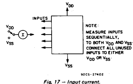
Fig. 17 - Input current.
