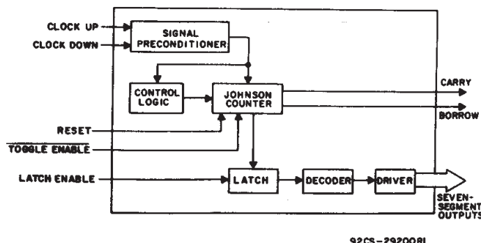
Fig. 1 - Functional diagram.
