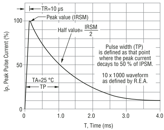
Pulse Rating Curve
