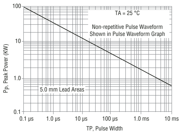
Pulse Rating Curve
