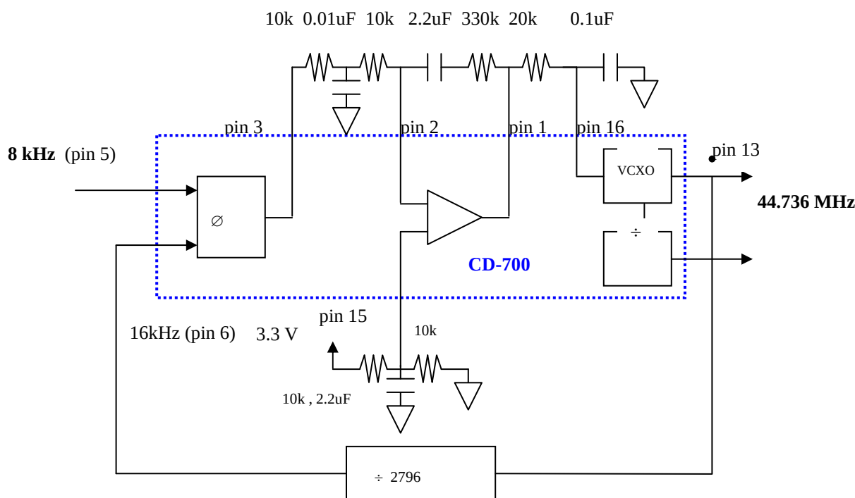
Figure 8. 8kHz to 44.736 MHz Frequency Translation
