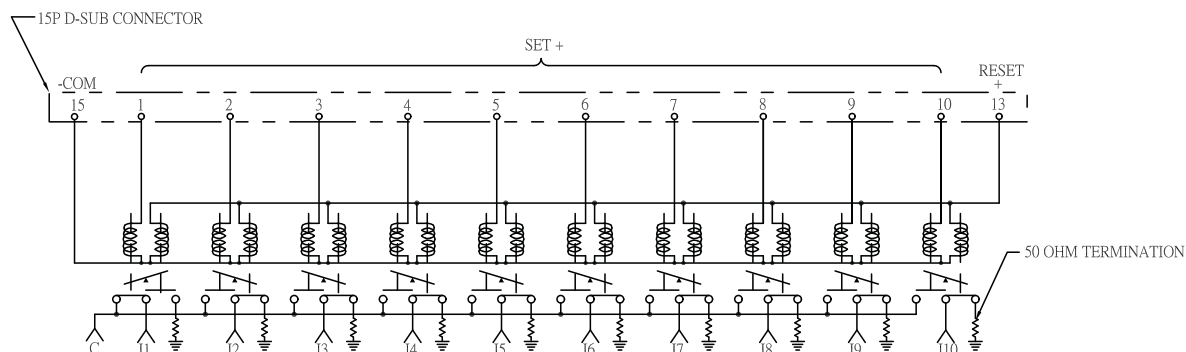
SCHEMATIC COIL 1 SHOWN LAST ENERGIZE
