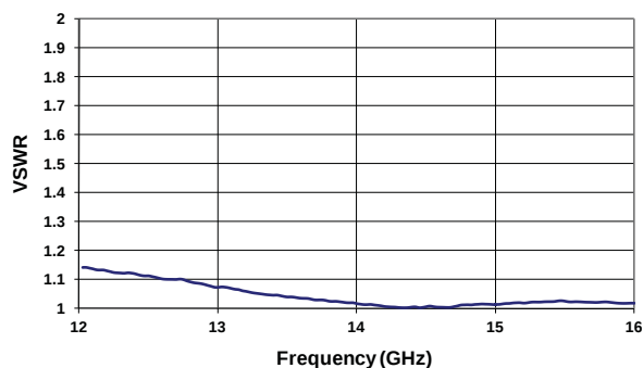
VSWR ( 12-16 GHz )
