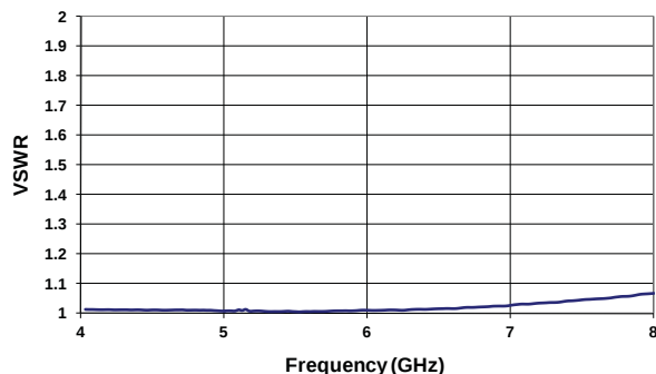
VSWR ( 4-8 GHz )
