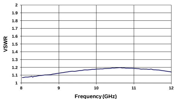
VSWR ( 8-12 GHz )
