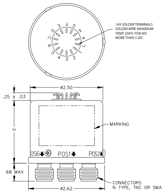
SP3T - SP6T H = 2.15 STD & Indicator Model SP3T - SP6T H = 2.65 All OTHER Models
