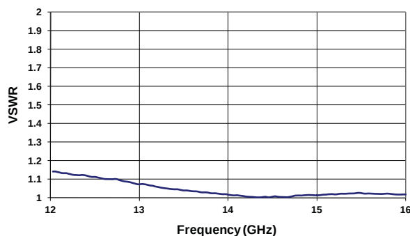
VSWR ( 12-16 GHz )
