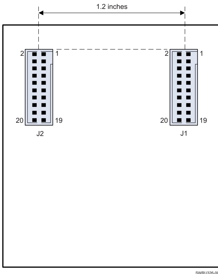
Figure 2-7. Host PCB Mating Connector Arrangement
