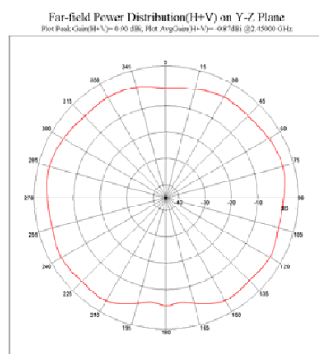
Figure 2-6. Antenna Radiation Patterns
