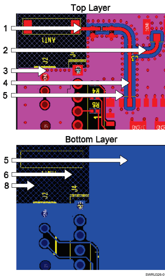
Figure 3-5. Antenna and RF Trace Routing Layout Guidelines
