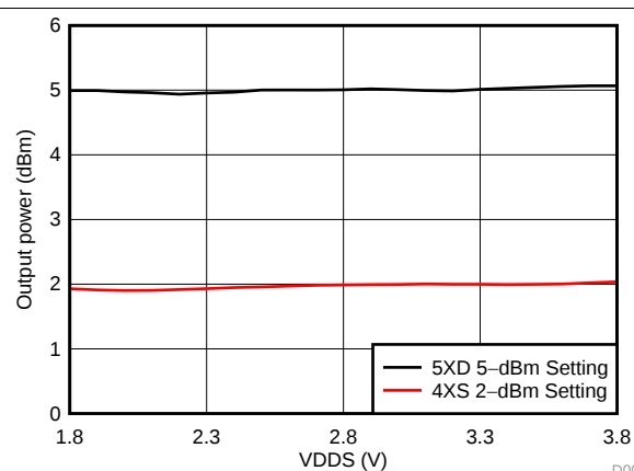
Figure 5-11. TX Output Power vs Supply Voltage (VDD5)
