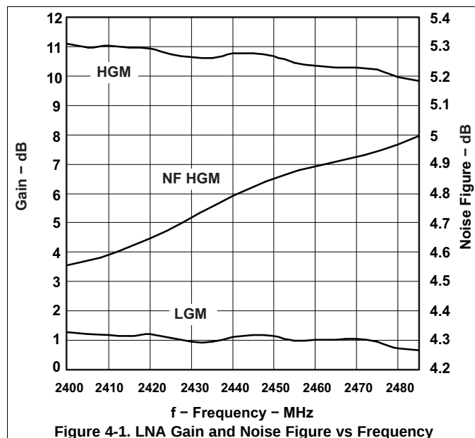
Figure 4-1. LNA Gain and Noise Figure vs Frequency
