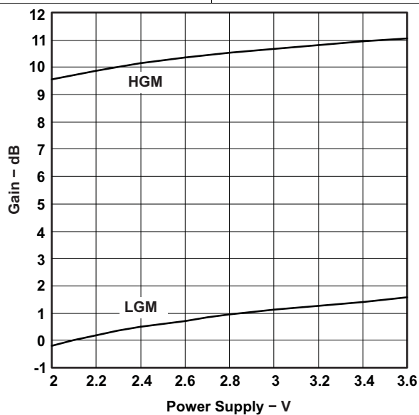
Figure 4-3. LNA Gain vs Power Supply
