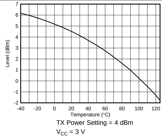
Figure 4-10. TX Power vs Temperature
