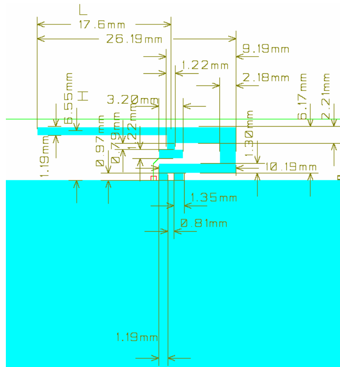
Figure 2: Antenna dimensions
