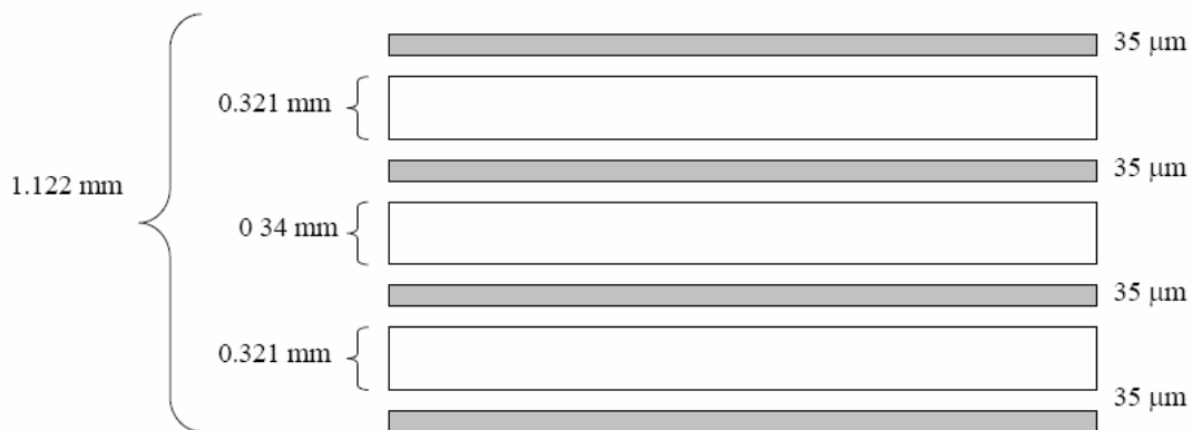
Figure 8: CC2420DB Layer Build Up
