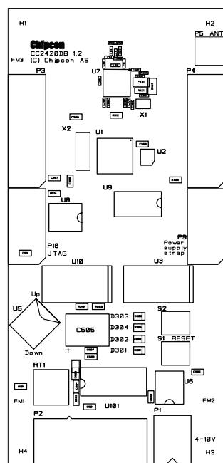
Top Assembly
