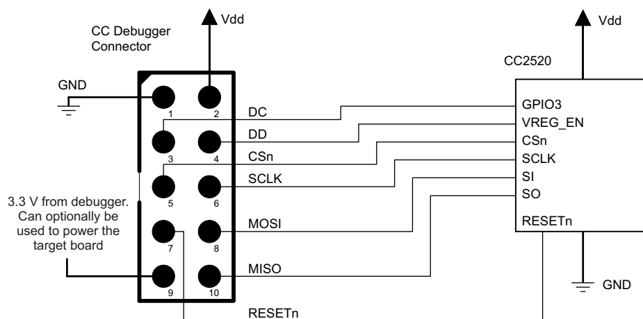
Figure 8. CC Debugger Connected to CC2520
