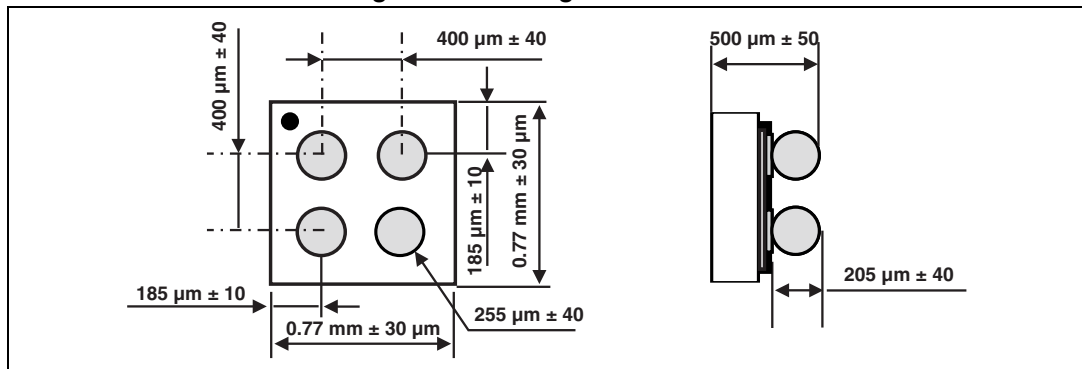
Figure 10. Package dimensions
