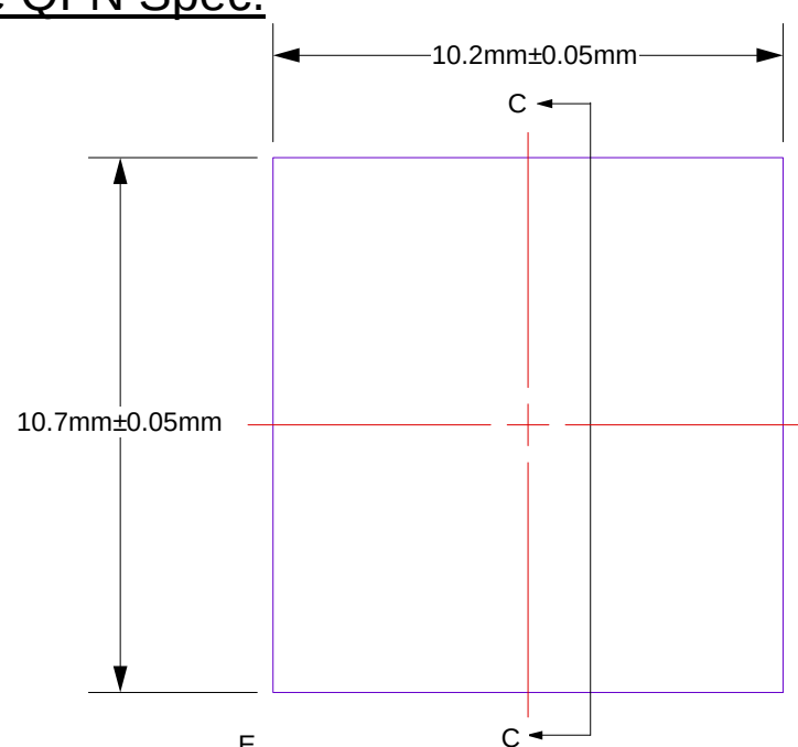
Top View
