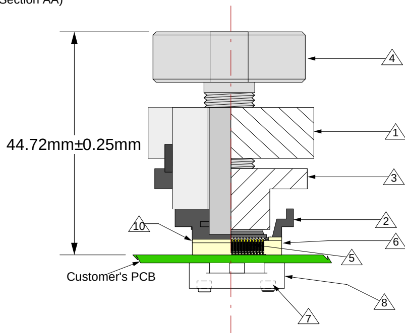
Side View (Section AA)
