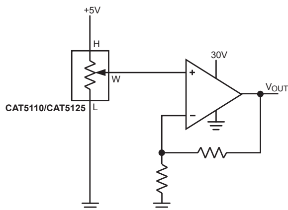
Figure 3. Positive LCD Bias Control
