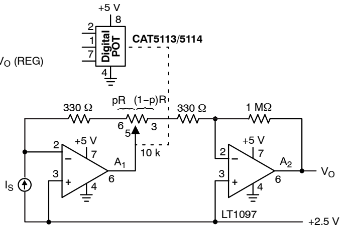
Figure 11. Programmable I to V Convertor
