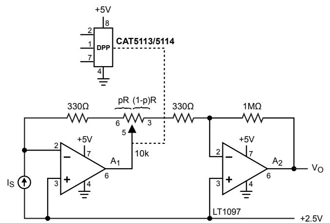
Programmable I to V Convertor
