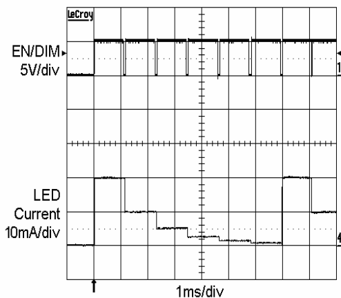
Dimming Waveform
