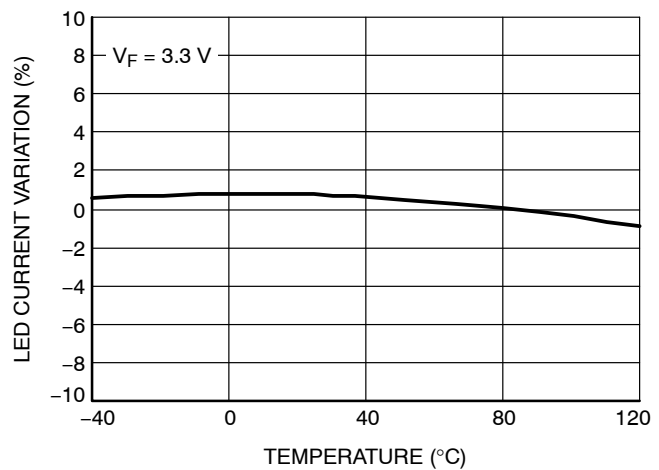
Figure 8. LED Current Change vs. Temperature
