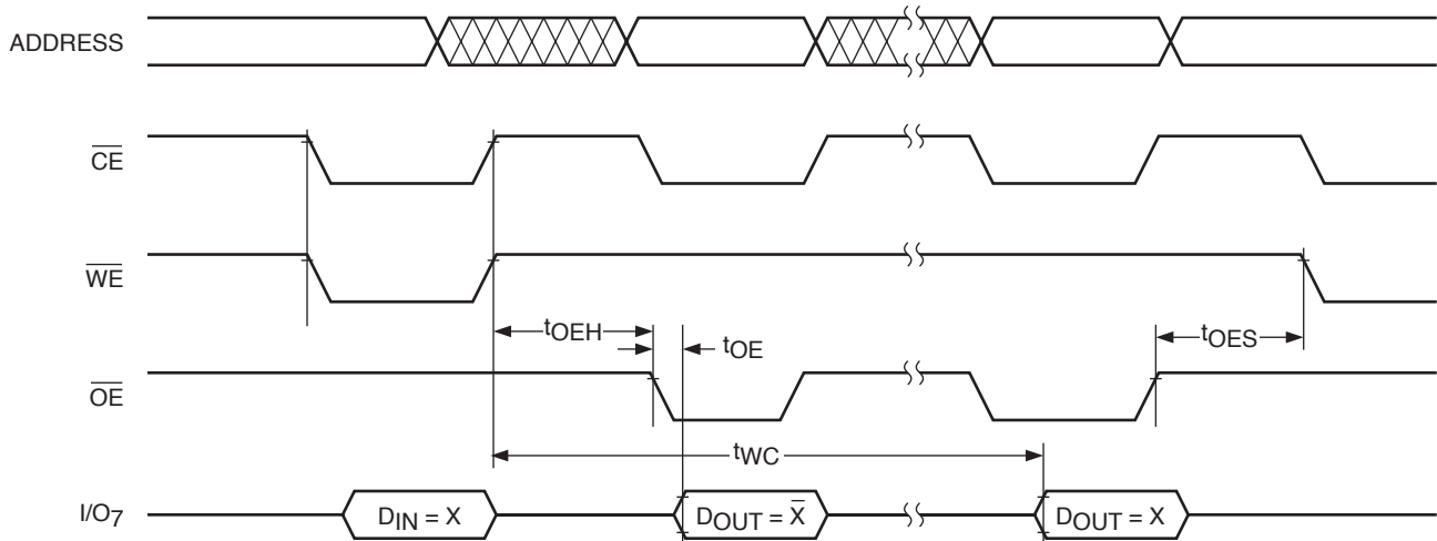
Figure 7. DATA Polling
