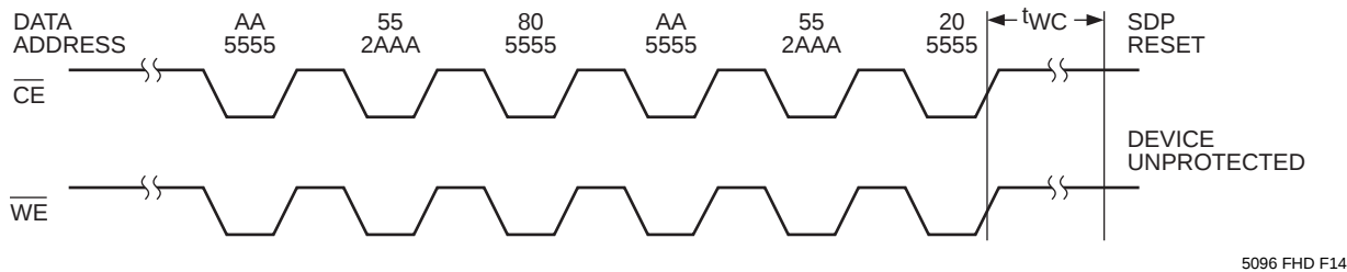
Figure 12. Resetting Software Data Protection Timing
