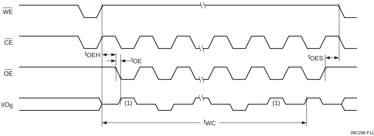
Figure 8. Toggle Bit
