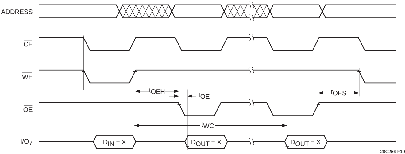
Figure 7. DATA Polling
