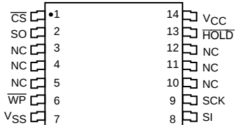
TSSOP Package (U14, Y14) SOIC Package (S, V)
