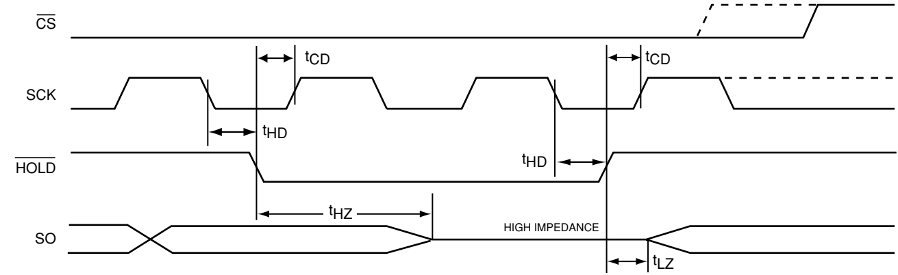
Figure 9. HOLD Timing
