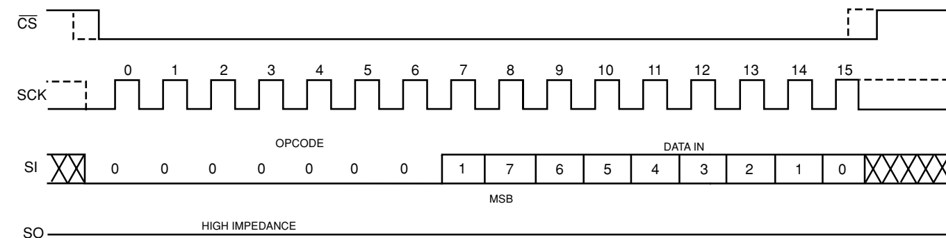
Figure 7. WRSR Timing
