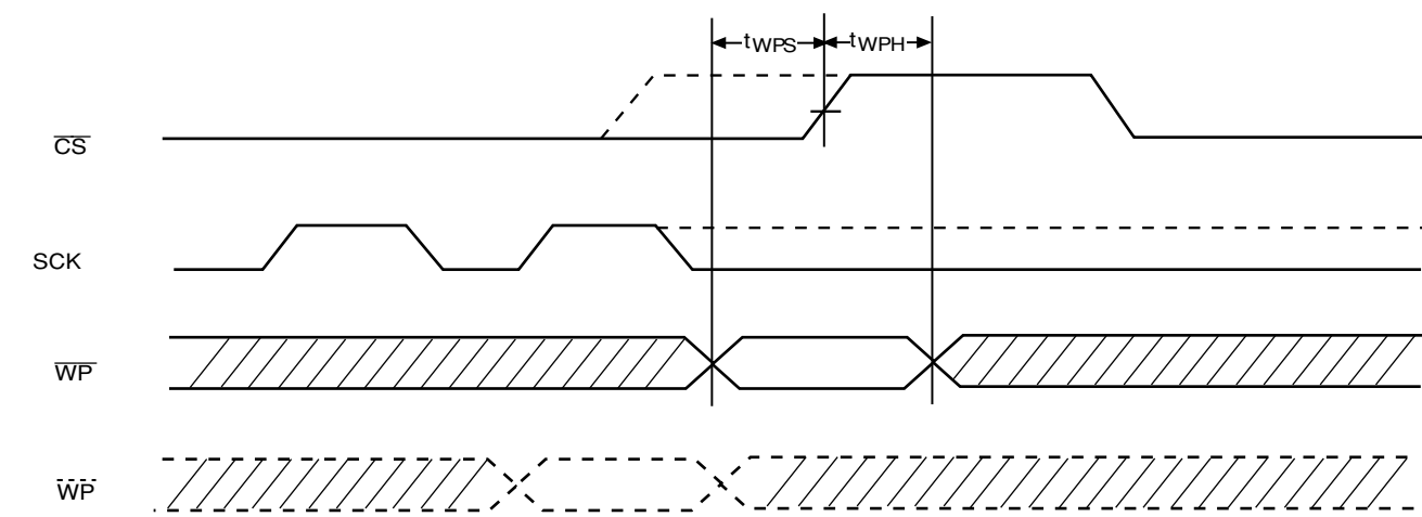
Figure 10. WP Timing
