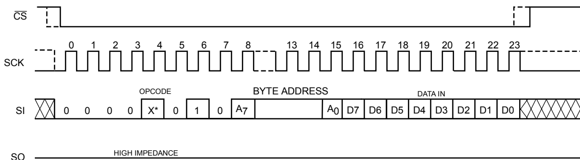
Figure 4. Byte WRITE Timing
