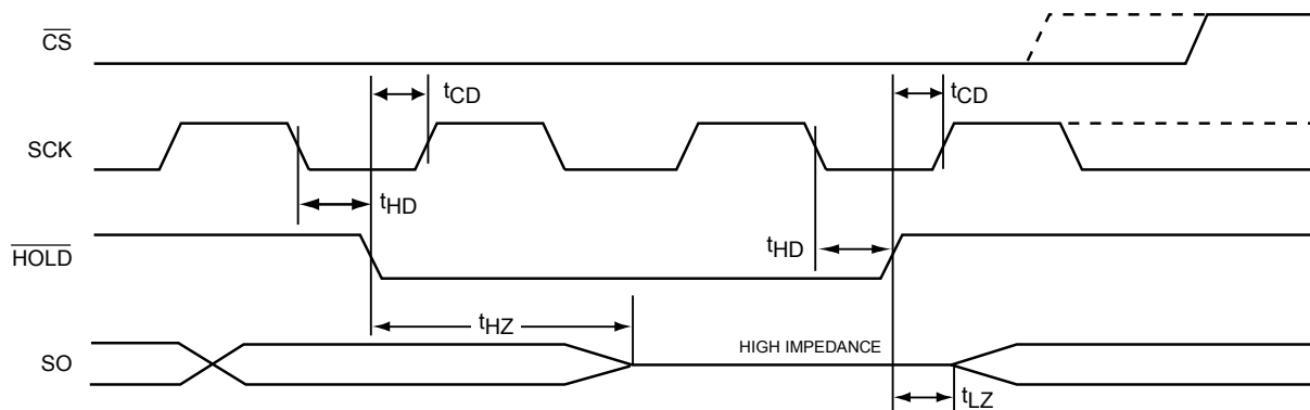
Figure 10. \overline{\text{HOLD}} Timing
