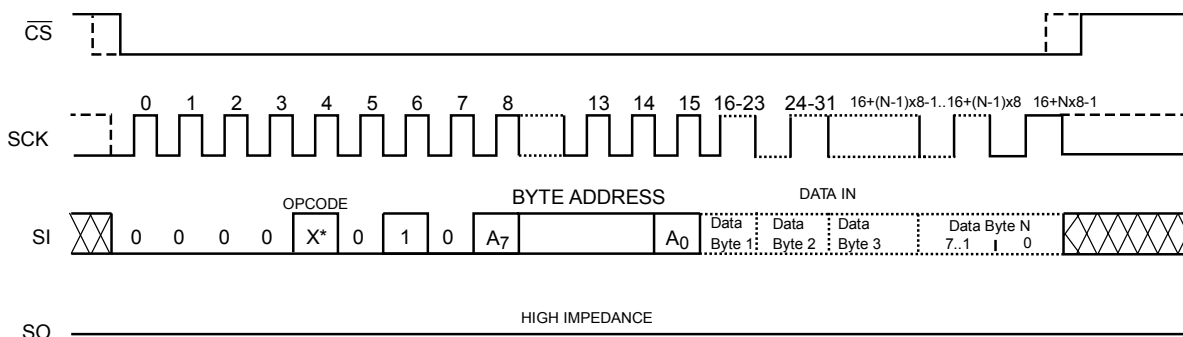
Figure 5. Page WRITE Timing
