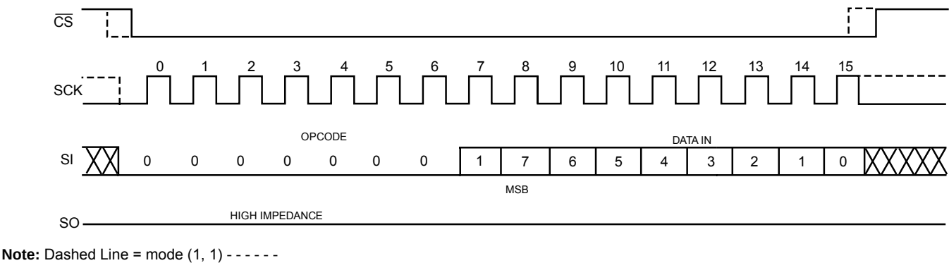
Figure 6. WRSR Timing
