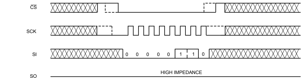
Figure 2. WREN Timing
