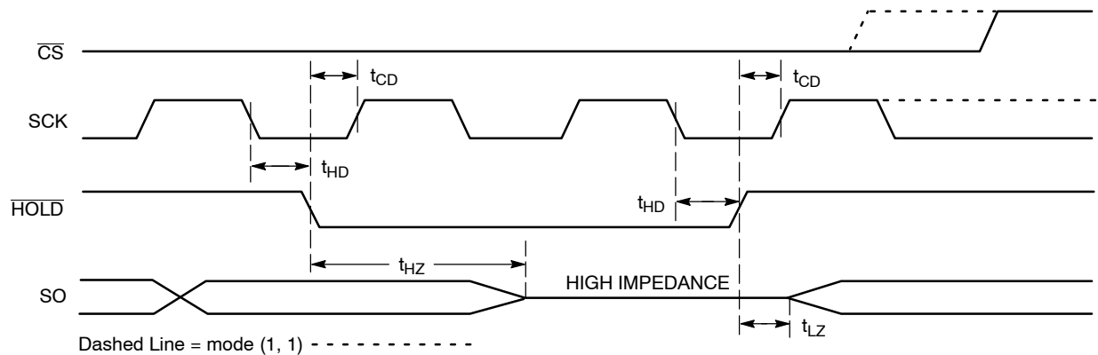
Figure 11. HOLD Timing
