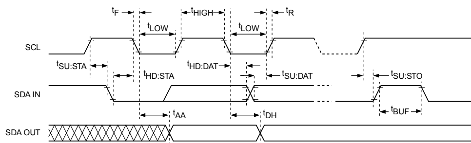
Figure 3. Bus Timing
