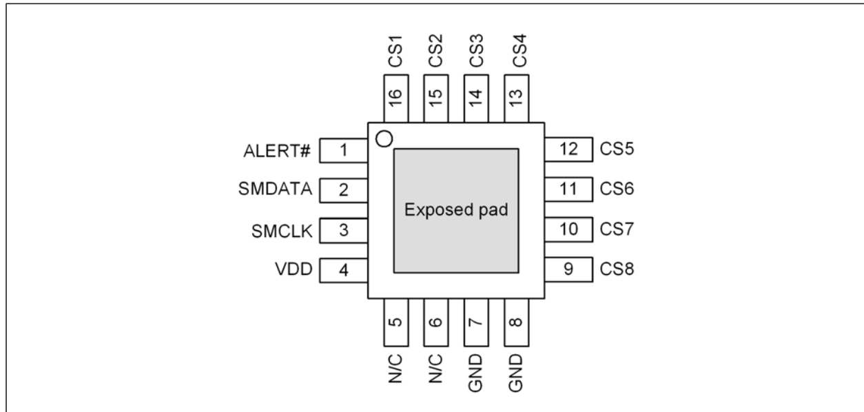
FIGURE 1-3: CAP1208 PIN DIAGRAM (16-PIN QFN)
