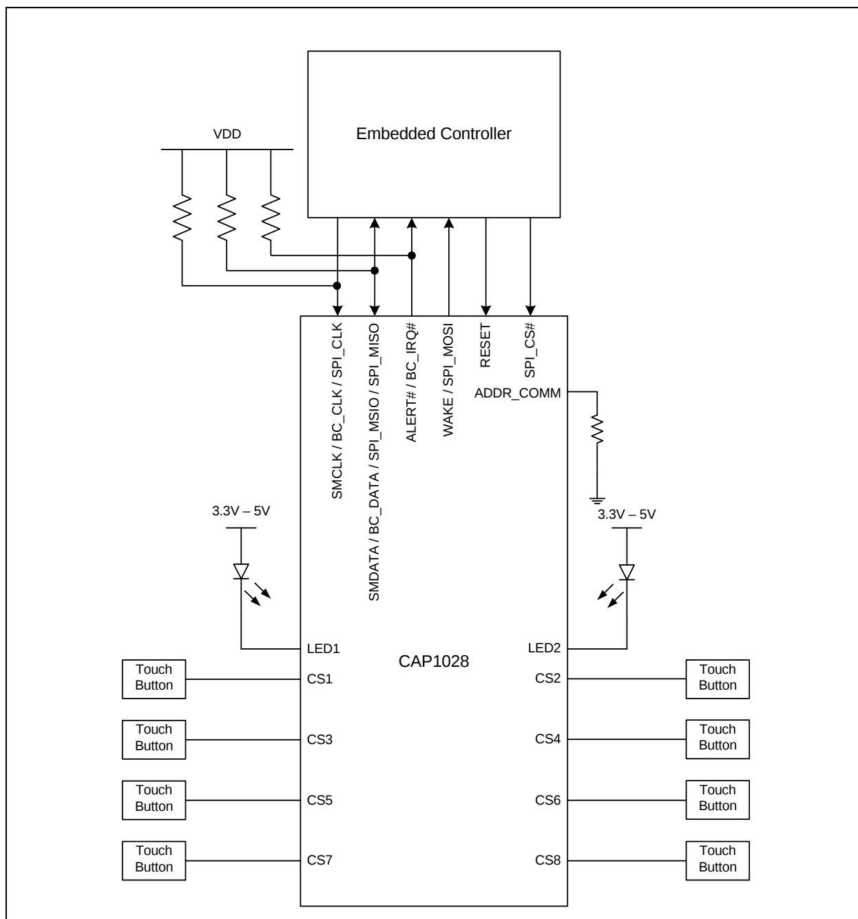
Figure 4.1 System Diagram for CAP1028
