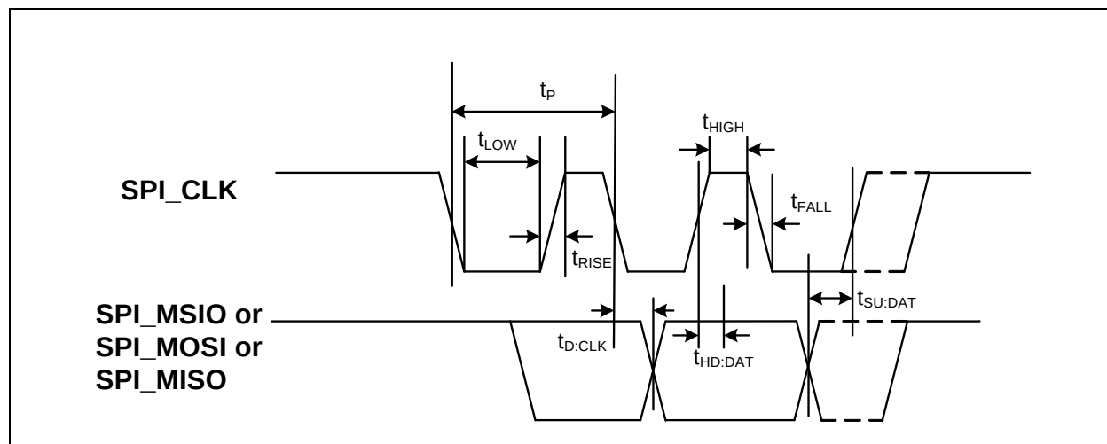
Figure 3.1 SPI Timing
