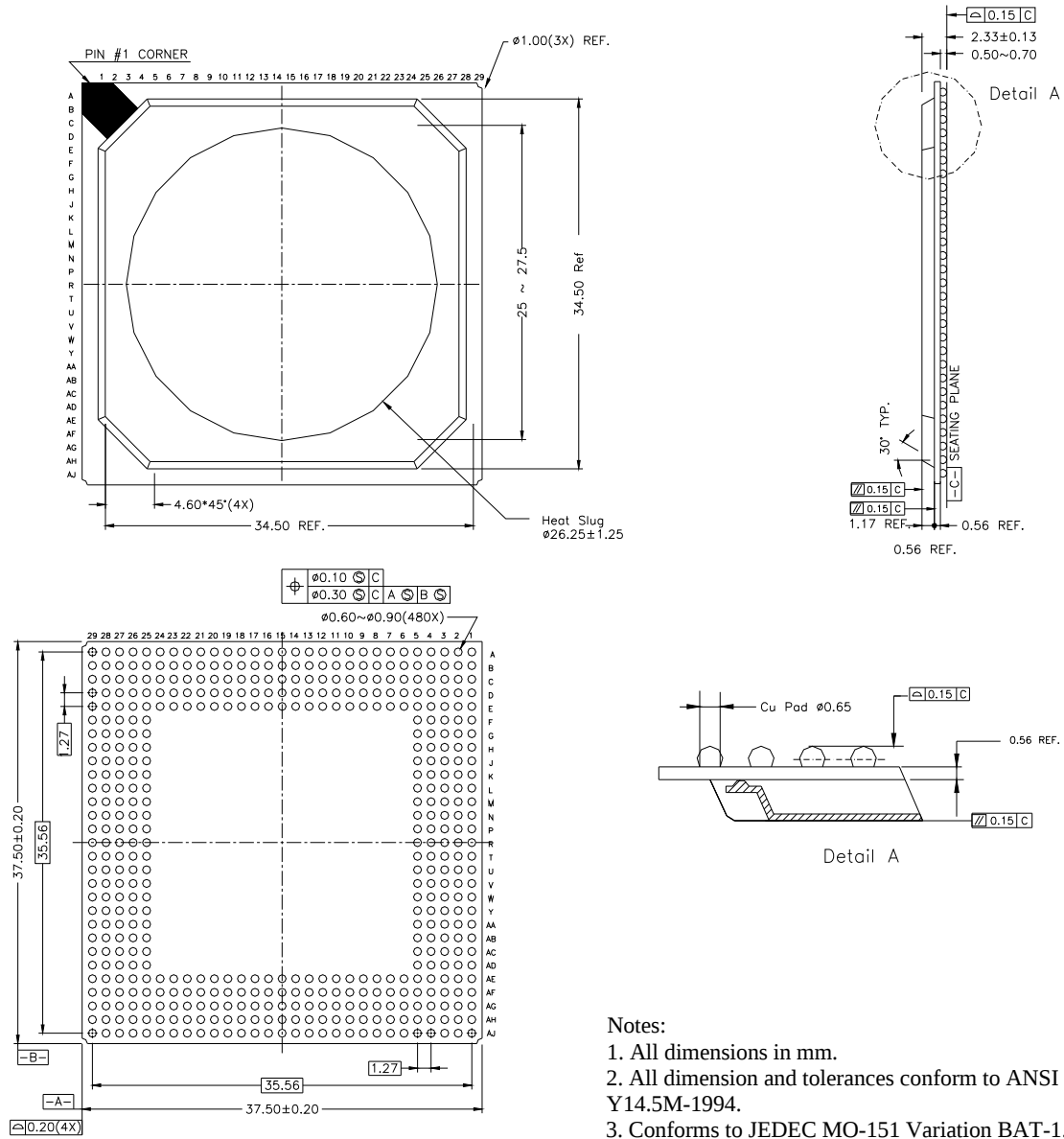
Figure 24: 480 HSBGA
