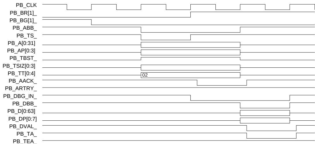
Figure 16: PB Master Interface Single Cycle Write
