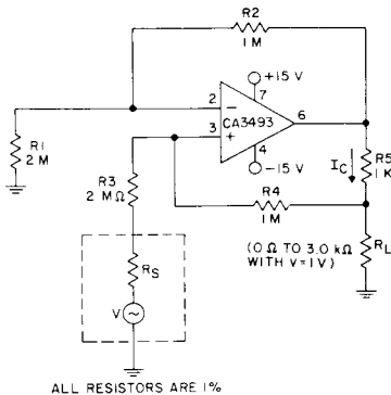
Fig. 20 - Typical two-op amp bridge-type differential amplifier.
