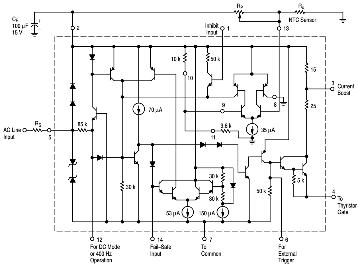
Figure 14. Circuit Schematic
