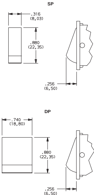
J6 FLAT ROCKER
