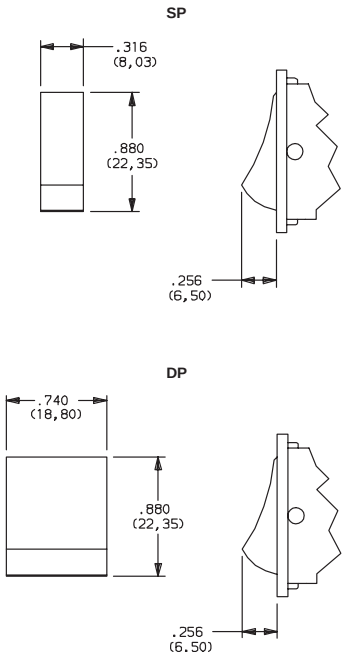
J7 CURVED ROCKER
