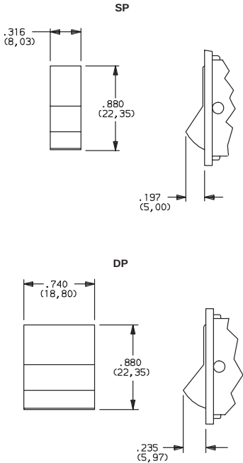
J1 (STD.) ROCKER
