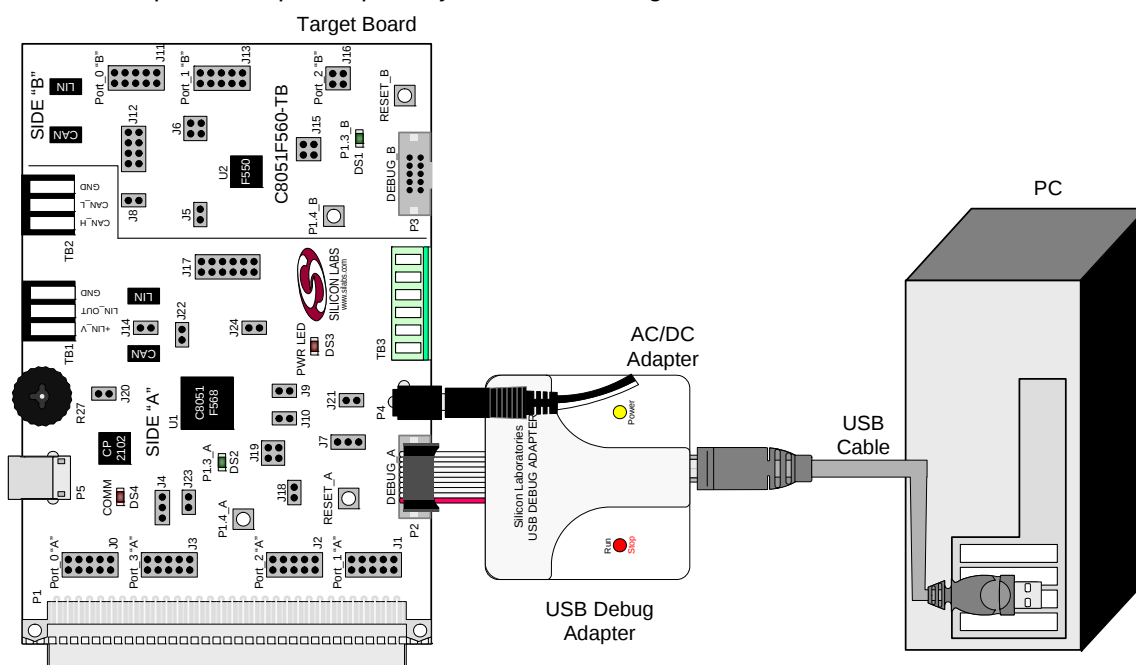
Figure 1. Hardware Setup using a USB Debug Adapter
