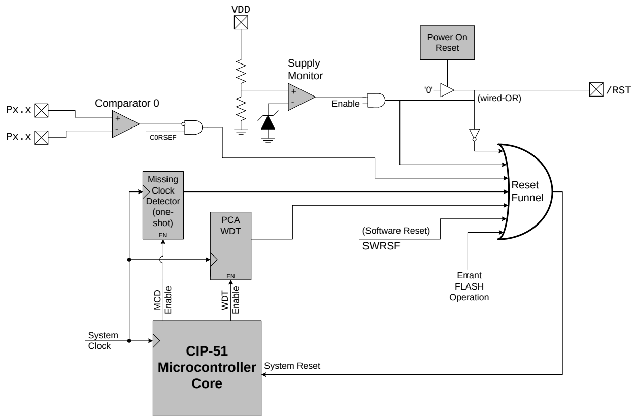
Figure 10.1. Reset Sources
