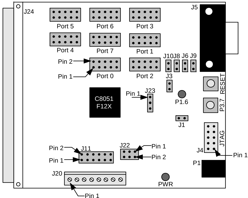
Figure 2. C8051F120 Target Board
