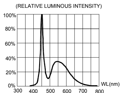
FIG.4 RELATIVE LUMINOUS INTENSITY VS. WAVELENGTH. 50% Power Angle : 105°
