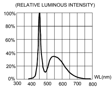
FIG.4 RELATIVE LUMINOUS INTENSITY VS. WAVELENGTH. 50% Power Angle : 105°
