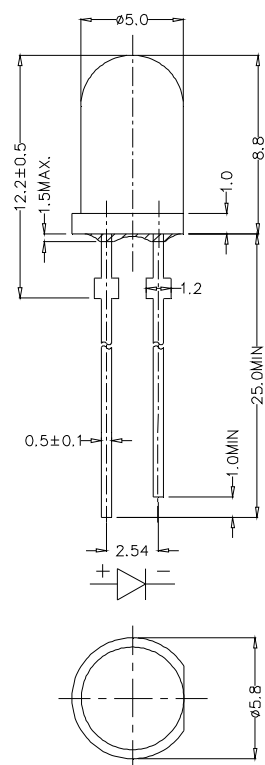
C503B-BCS/GCS:
