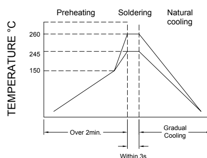
Figure 2. Wave Soldering
