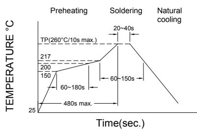
Figure 1. Re-flow Soldering
