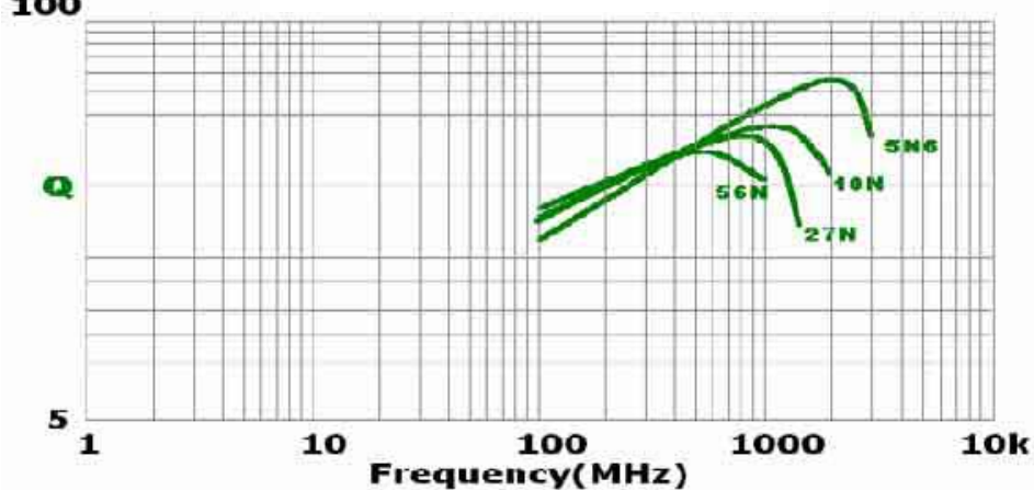
Q vs. Frequency Characteristics
