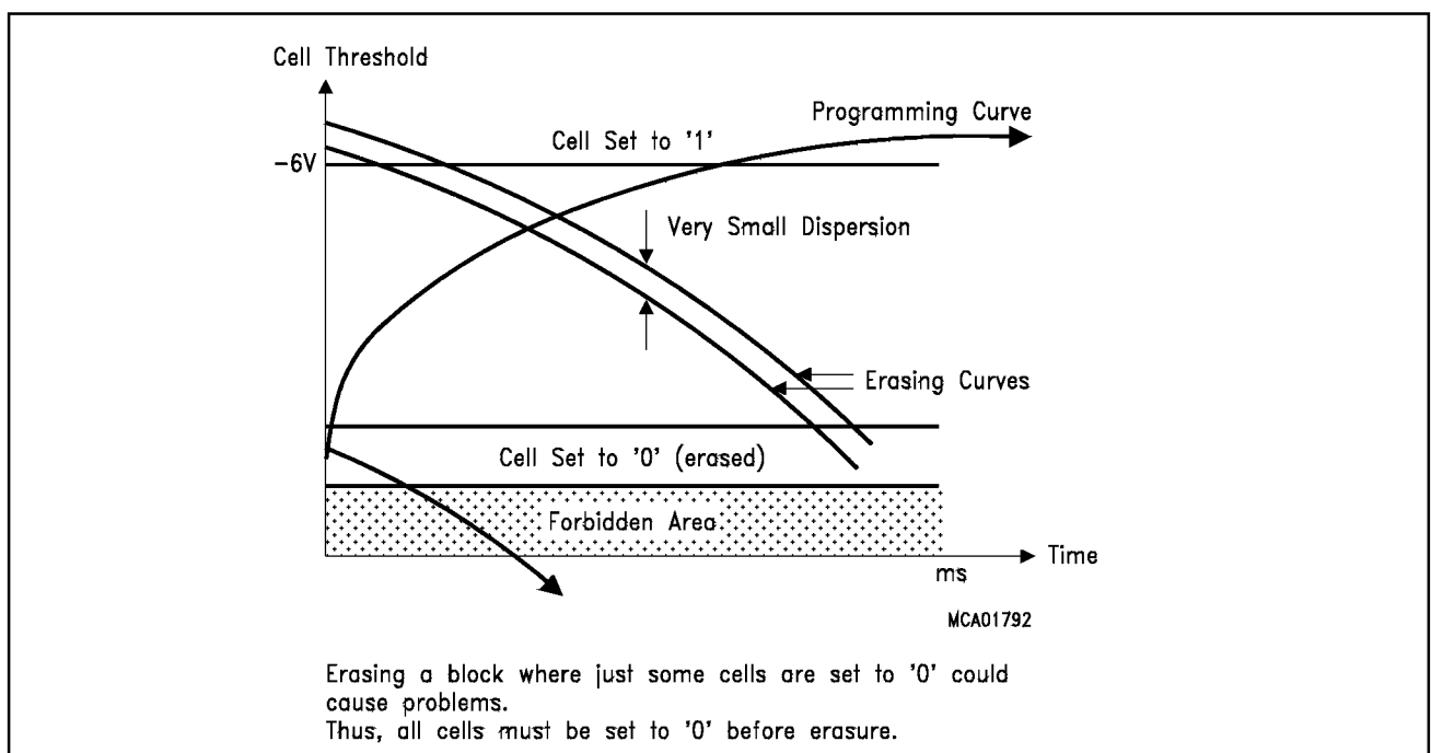
Figure 11 Flash Erasure
