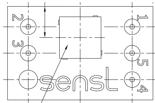
Figure 11. MicroFC-SMTPA-XXXXX
